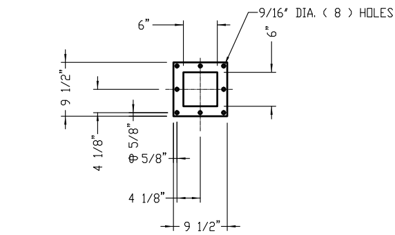
VIEW A-A INLET FLANGE
